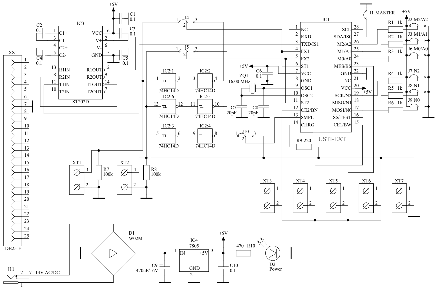
Figure 11. The USTI-EXT Development Board Circuit Diagram.
