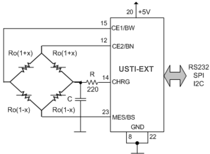
Figure 10. The USTI-EXT Circuit Diagram for Resistive Bridge Measurement.
