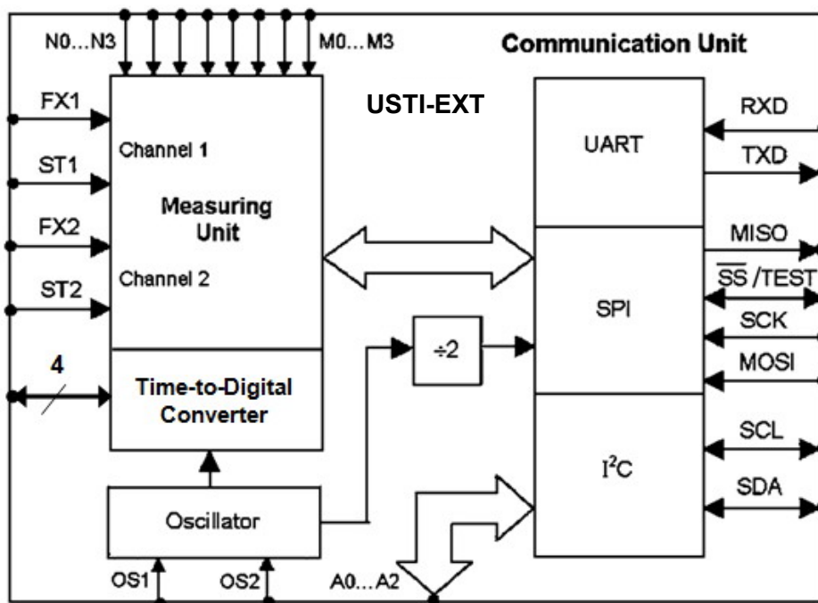
Figure 1. The USTI-EXT Block Diagram.
