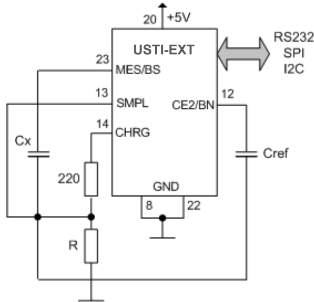
Figure 9. The USTI-EXT Circuit Diagram for Capacitance Measurement.
