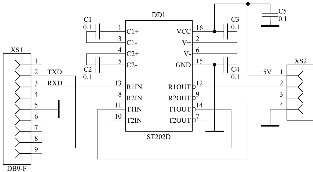
Figure 5. Interfacing Circuit for Connection the USTI-EXT to PC.
