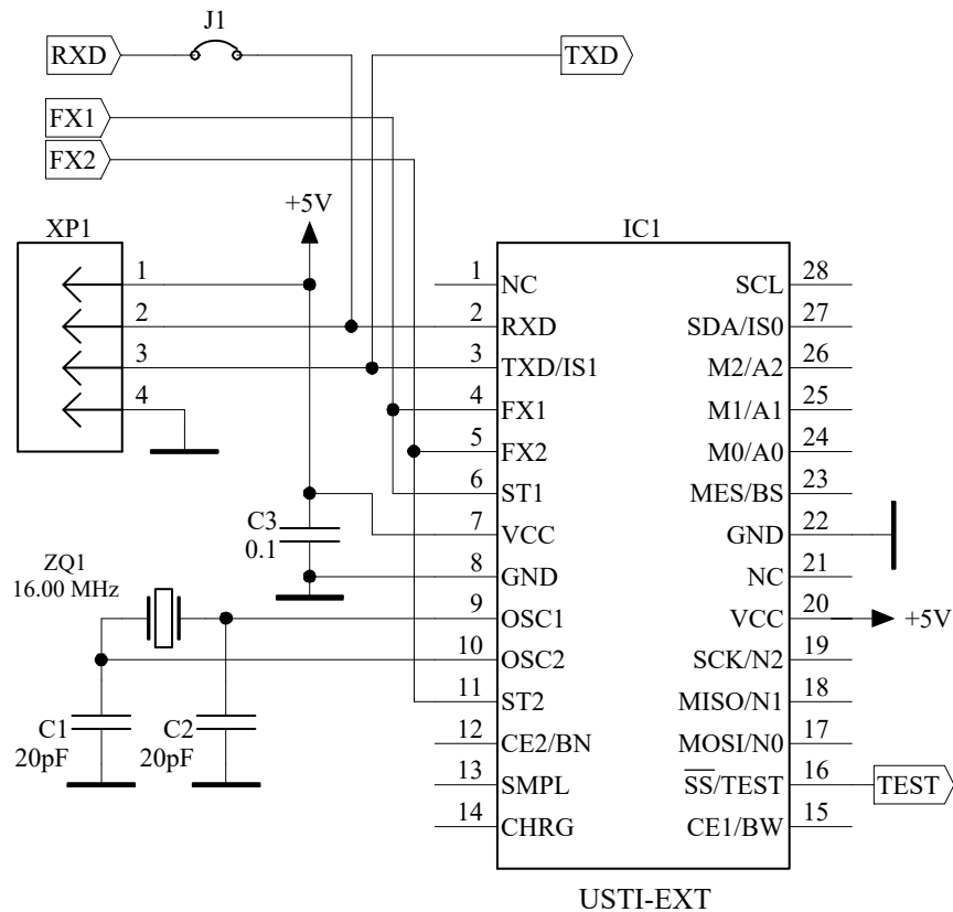
Figure 4. Circuit Diagram for the USTI-EXT Working Embedded in a Sensor or DAQ Board (Slave Mode).
