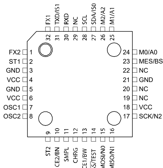
Figure 2. Pin Configuration and Housing (Not to Scale). NOTE: Bottom Pad for MLF Package Should be Soldered to Ground.
