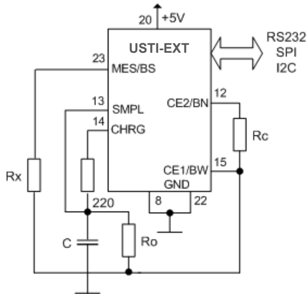
Figure 8. The USTI-EXT Circuit Diagram for Resistance Measurement.
