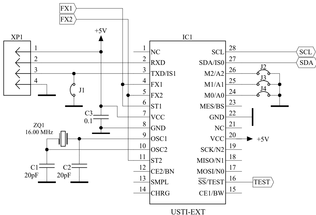
Figure 7. The USTI-EXT Circuit Diagram for the 2-wire I 2 C Interface.
