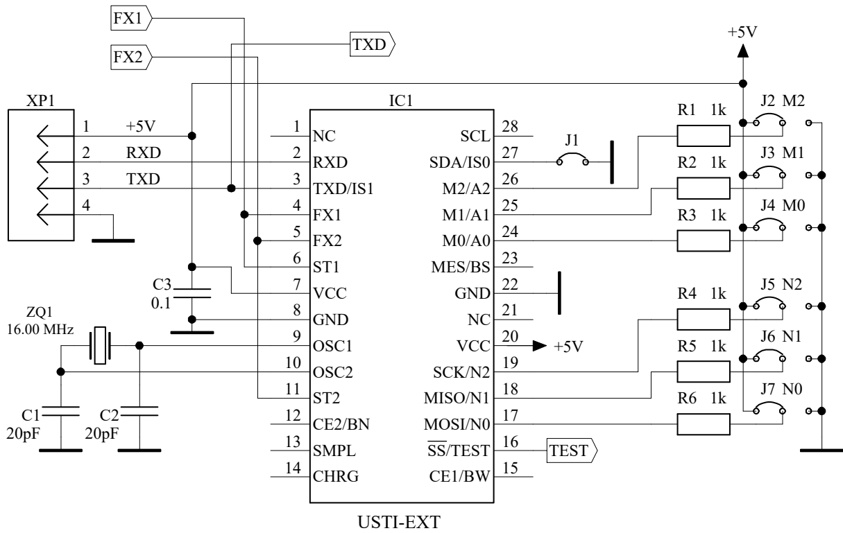
Figure 3. Circuit Diagram for the USTI-EXT Working in Autonomous (Master) Mode, RS232 Interface.
