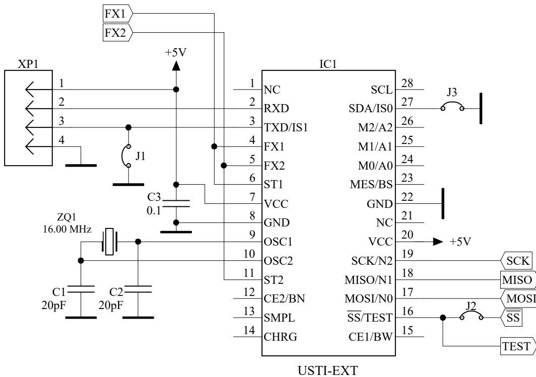
Figure 6. The USTI-EXT Circuit Diagram for the 3-wire Serial Interface (SPI).
