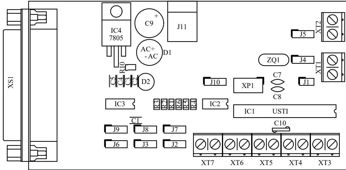
Figure 12. The USTI-EXT Development Board Silkscreen (Not to Scale).
