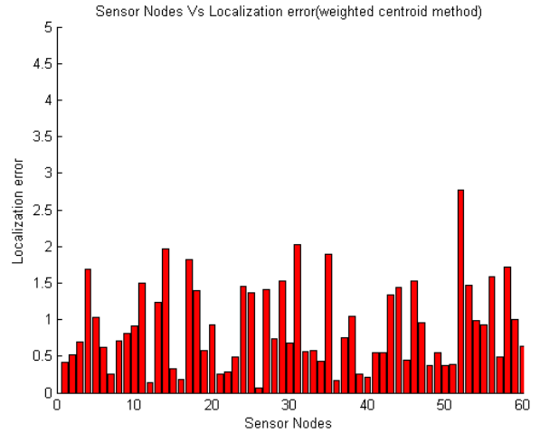
Fig. 9. Error Results (Weighted Centroid Method).
