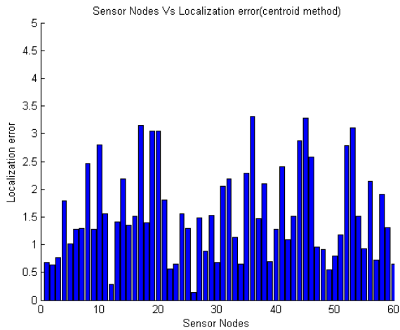
Fig. 8. Error Results (Centroid Method).
