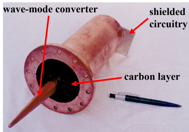
Fig. 9. Waveguide-fitted calorimetric sensor.
