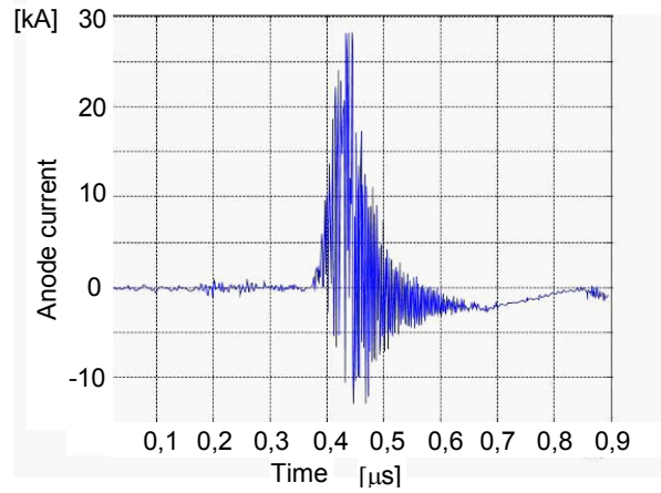
Fig. 7. Waveform of vircator's anode current.
