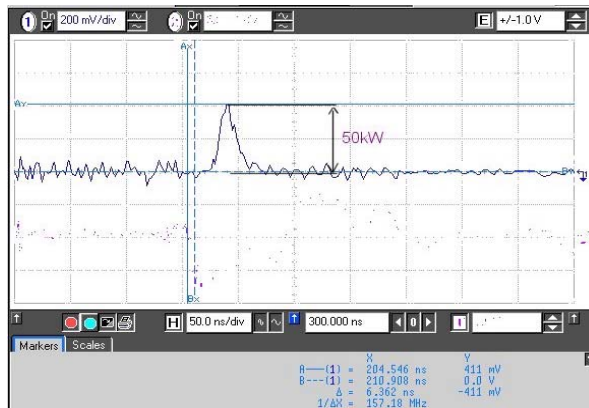
Fig. 15. Measured waveform of small microwave power, P_{\max} = 50 kW.
