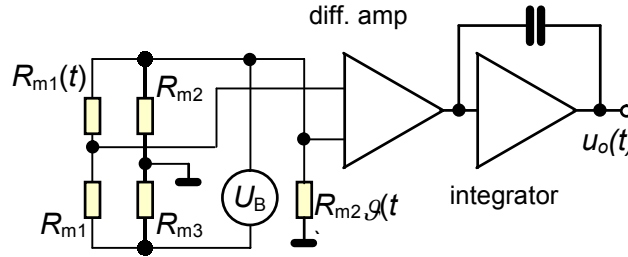
Fig. 10. Principle scheme of the sensor circuitry.
