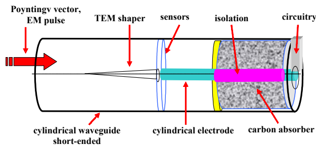
Fig. 8. Principal scheme of the calorimetric sensor.
