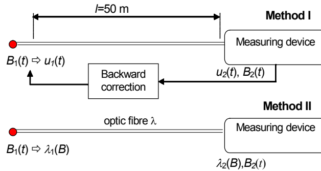
Fig. 2. Principles of the methods based on Faraday’s induction law and magneto-optic effect.
