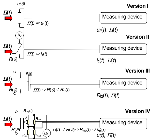
Fig. 5. Calorimetric measurement of the solitary pulse power.
