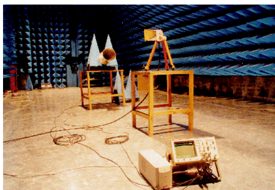
Fig. 14. Calibration of the calorimetric sensor.
