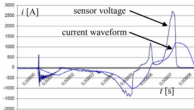
Fig. 4. Example of the current pulse waveform.
