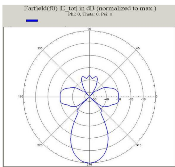
Fig. 13. Radiation pattern of Horn-type antenna in dB.
