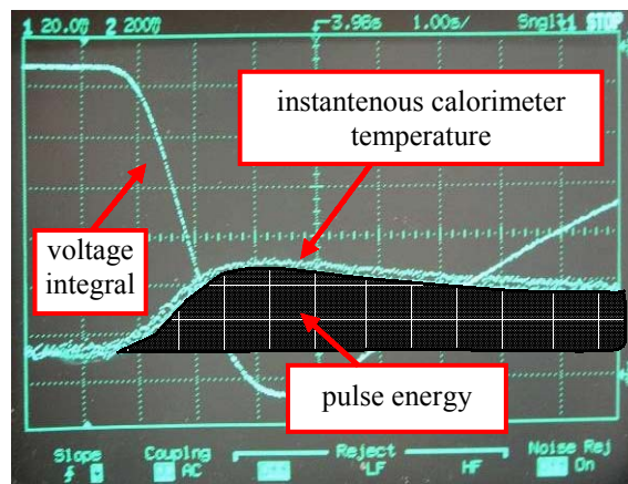
Fig. 11. The output voltage of the calorimeter and its integral.
