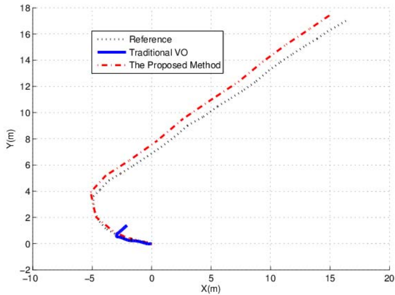
Fig. 5. Experiment 2, camera position estimation for an image sequence captured in real-world scenes. There is an independently moving object in the scenes for frame 18 to 27.
