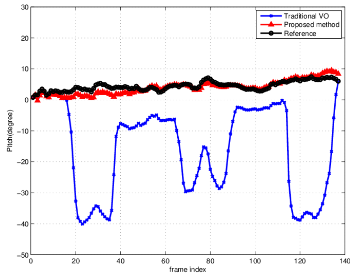
Fig. 7. Experiment 3, camera orientation (pitch) estimation for an image sequence captured in real-world scenes.
