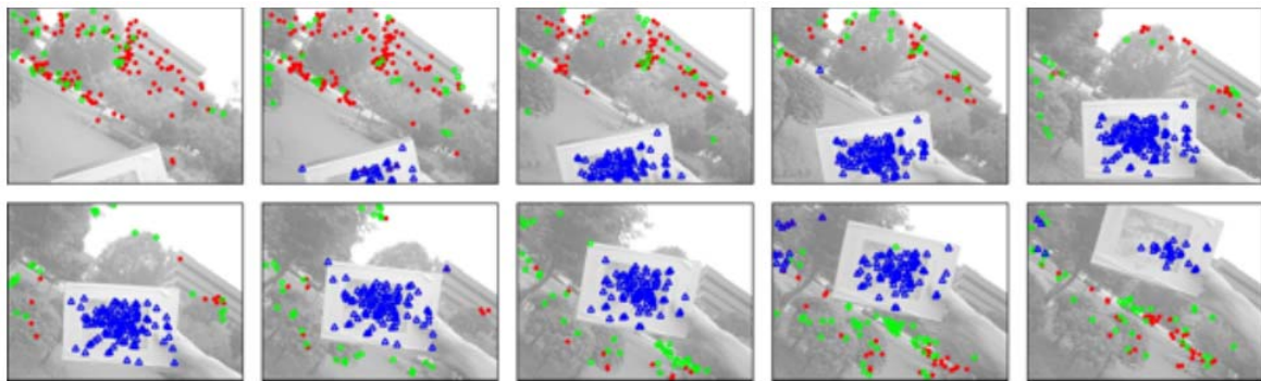
Fig. 3 Background Model Updating Process. Markers of hollow green circles are "fresh" background feature points, markers of solid red circles are matching background points and blue triangles are foreground points.
