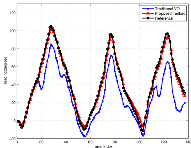
Fig. 6. Experiment 3, camera orientation estimation (heading) for an image sequence captured in real-world scenes.
