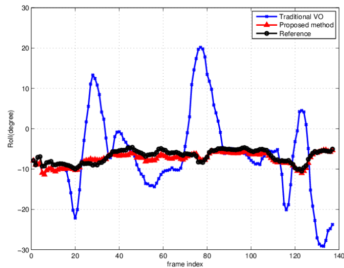
Fig. 8 Experiment 3, camera orientation (roll) estimation for an image sequence captured in real-world scenes.
