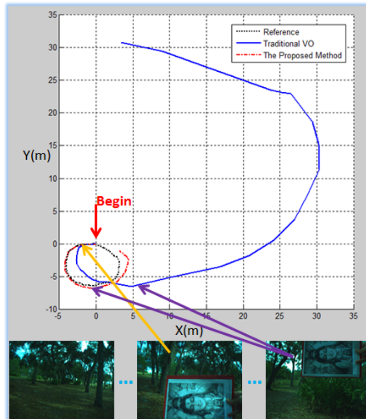
Fig. 4. Experiment 1, camera position estimation for an image sequence captured in real-world scenes. There is an independently moving object in the scenes for frame 23 to 31 and frame 108 to 115.
