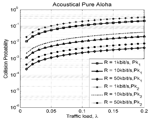
Fig. 6. Collision Probability of Acoustic pure ALOHA with different traffic load \lambda and packet data dimensions.
