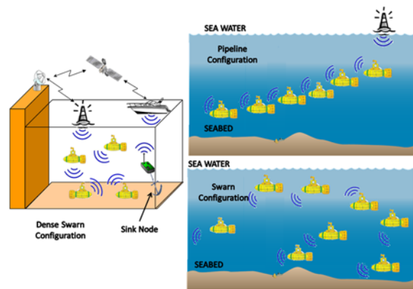
Fig. 1. Typical Underwater Swarm Configurations: the Dense Swarm Case (on the left side of the picture), the Pipeline Case (on the upper right side of the picture) and a combination of them, the Swarm Case (on the lower right side of the picture).
