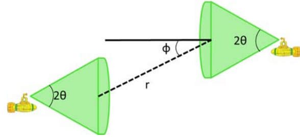
Fig. 2. Optical Channel characterization: half transmitter-receiver beam width ( \theta ), and the angle between the receiver optical axis and the line-of-sight between transmitter and receiver ( \Phi ).
