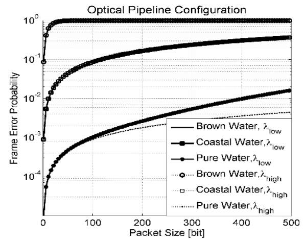
Fig. 11. Frame Error Probability versus packet size with optical channel and Slotted Aloha MAC (Pipeline Case).
