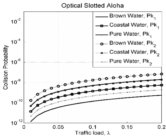
Fig. 9. Collision Probability of Optical Slotted ALOHA with different traffic load \lambda and packet data dimensions.
