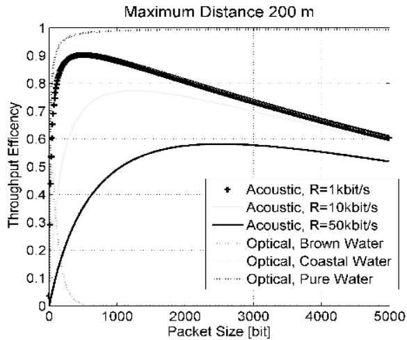
Fig. 5. \eta of S&W vs packet size N_d for acoustic (different data rates) and optical (different water) technologies: at the maximum distance of 200 m.
