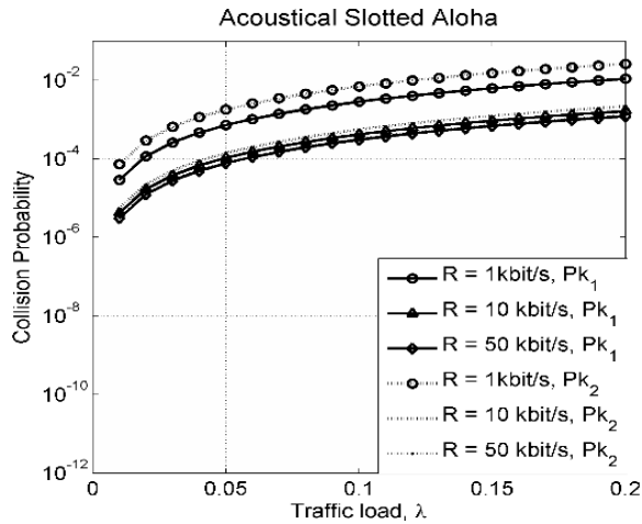
Fig. 8. Collision Probability of Acoustic Slotted ALOHA with different traffic load \lambda and packet data dimensions.
