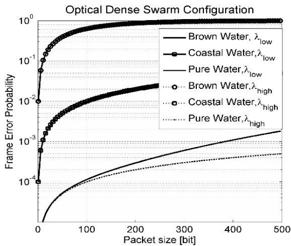
Fig. 13. FEP versus packet size with Optical channel and Slotted Aloha MAC (Dense Swarm Case).
