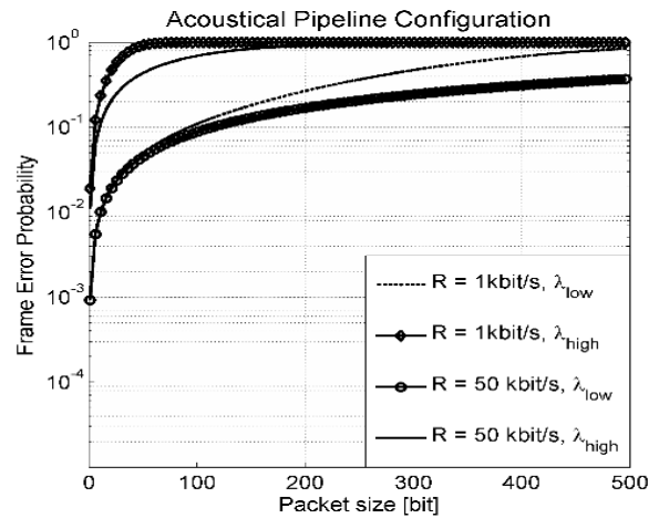
Fig. 10. Frame Error Probability versus packet size with acoustic channel and Slotted Aloha MAC (Pipeline Case).
