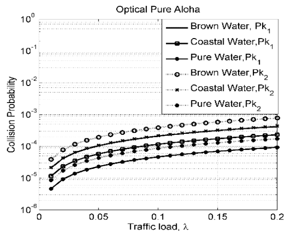
Fig. 7. Collision Probability of Optical pure ALOHA with different traffic load \lambda , and packet data dimensions.
