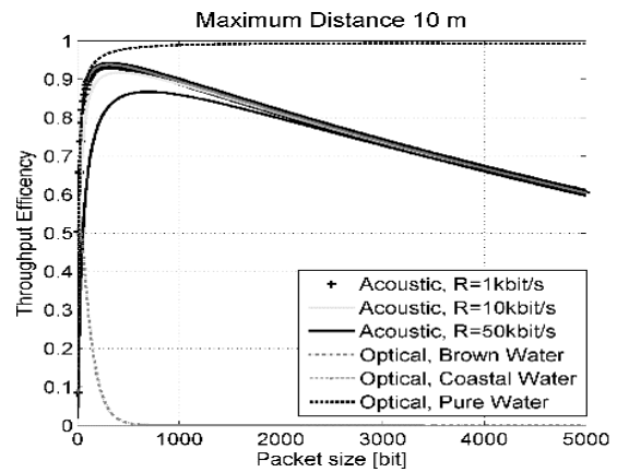
Fig. 4. \eta of S&W vs packet size N_d for acoustic (different data rates) and optical (different water) technologies :at the maximum distance of 10 m.
