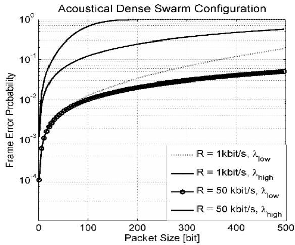
Fig. 12. FEP versus packet size with Acoustic channel and Slotted Aloha MAC (Dense Swarm Case).
