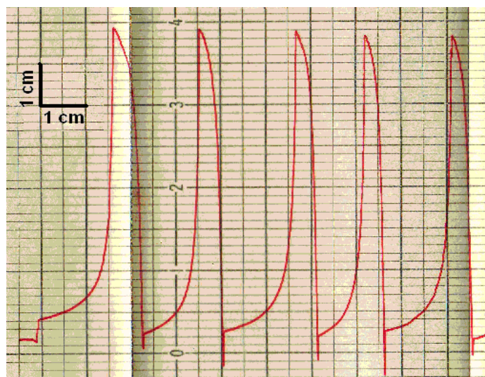
Fig. 2. Humidity sensor reproducibility; Cycled between two humidity levels. (Scale X-axis 1 min \text{cm}^{-1} and Y-axis 2.0 \text{mS cm}^{-1} ).
