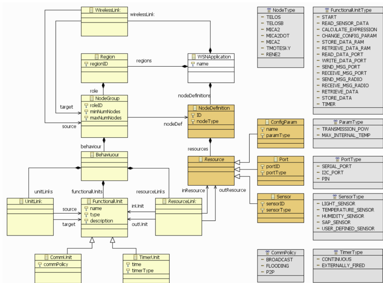
Fig. 13. WSN-DSL Meta-Model, reproduced from [2].
