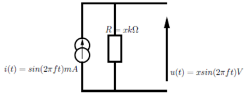
Fig. 18. Electronic Model of the Thermal Sensors [16].
