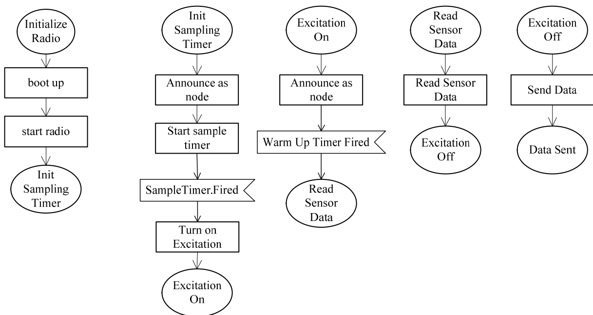
Fig. 5. SensIV SDL Process Diagram.
